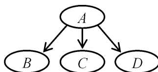
Figure 1. Multiple support for a hypothesis.
