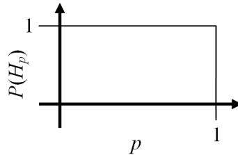
Figure 7. Uniform prior P(H_p) .
