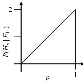
Figure 8. One head in one trial observed.
