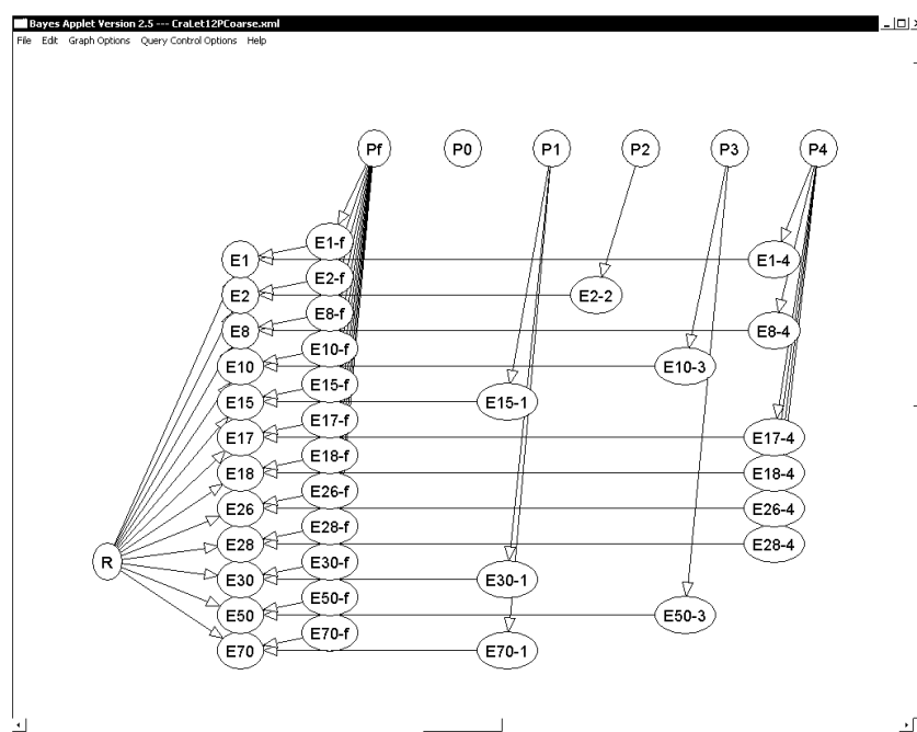
Figure 10. Network for twelve selected papers (initial configuration).
