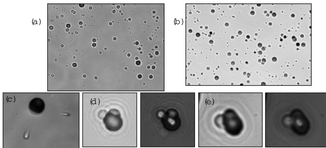
Figure 11. (a) Tracks on the backside of a CR-39 detector used in a Pd/D co-deposition experiment. (b) Tracks in CR-39 caused by neutrons from a ^{238}\text{Pu} fission source. (c) Results of sequential etching showing deeper proton recoil tracks. The black, 50\ \mu\text{m} diameter track on top is a surface track. Triple tracks obtained as a result of (d) Pd/D co-deposition and (e) exposure to DT neutrons. Left hand images in (d) and (e) obtained with the microscope optics focused on the surface of the detector. Right hand images in (d) and (e) are an overlay of two images taken at two different focusing depths (surface and bottom of the tracks). (c) and (d) reprinted with permission from Naturwissenschaften [29].
