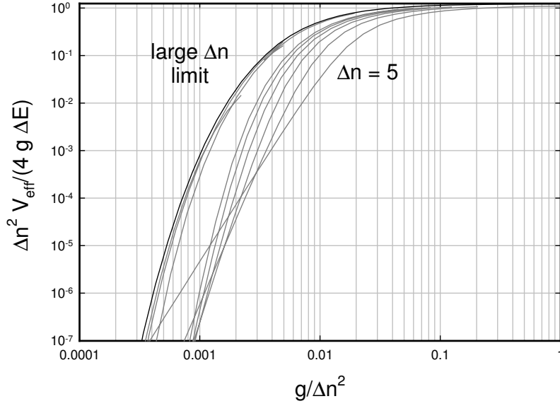
Figure 1. Scaled indirect coupling matrix element as a function of the scaled dimensionless coupling parameter g for different odd \Delta n , including 5, 7, 9, 11, 15, 51, 101, 151 (grey); also shown is the large \Delta n limit (black).
