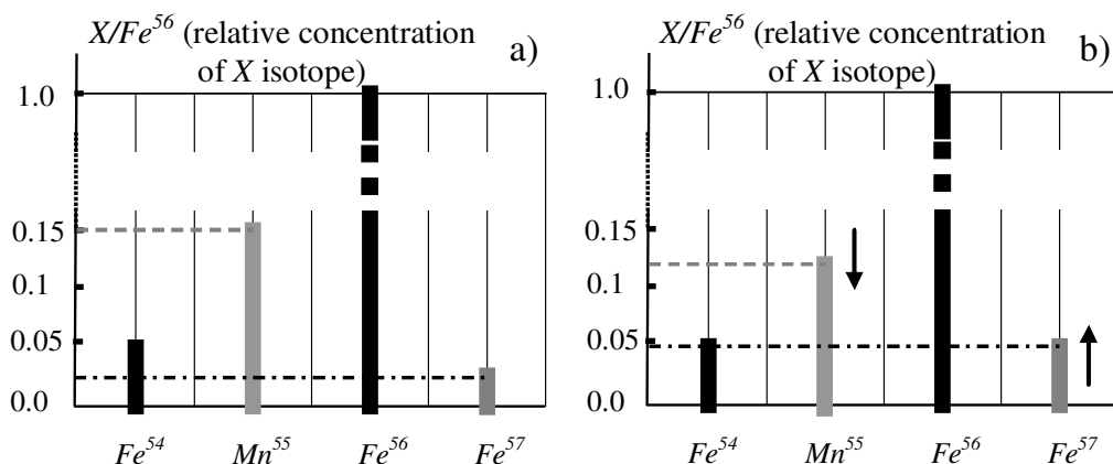
Figure 5. Mass-spectrum of iron-region of microbiological associations (dried biological substances) that were grown in control nutrient medium with H_2O and Mn^{55} (case a) and in experimental nutrient medium with D_2O and the same quantity of Mn^{55} isotope (case b). Here X = Fe^{54} ; Mn^{55} ; Fe^{57} . The process of increasing ( \uparrow ) concentration of Fe^{57} isotopes is accompanied by decreasing ( \downarrow ) concentration of Mn^{55} isotopes.
