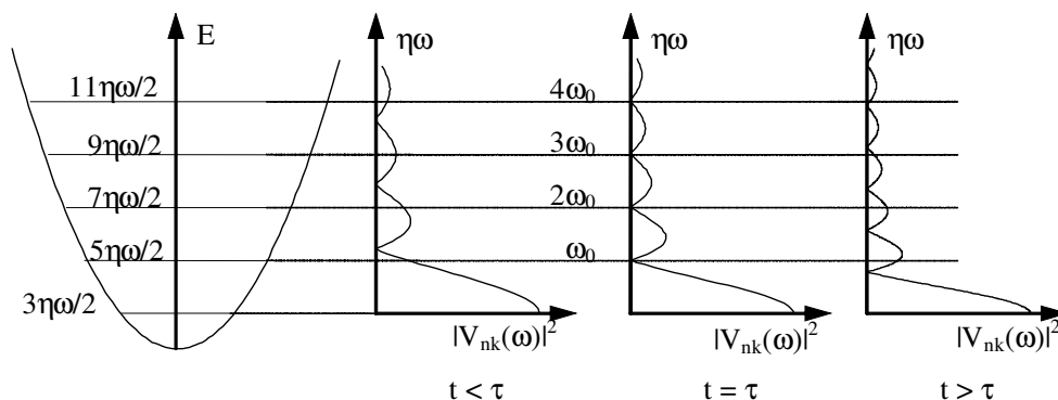
Figure 11. Correlation between energy spectrum of quantum levels E_n and spectral density |V_{nk}(w)|^2 of perturbation energy V(r) for short ( t < \tau ), optimal ( t = \tau ) and long ( t > \tau ) duration of \text{Mn}^{55} - \text{d}^2 nuclear interaction.
