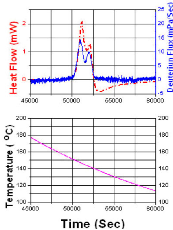
Figure 11. Correlation between heat flow and deuterium flux.
