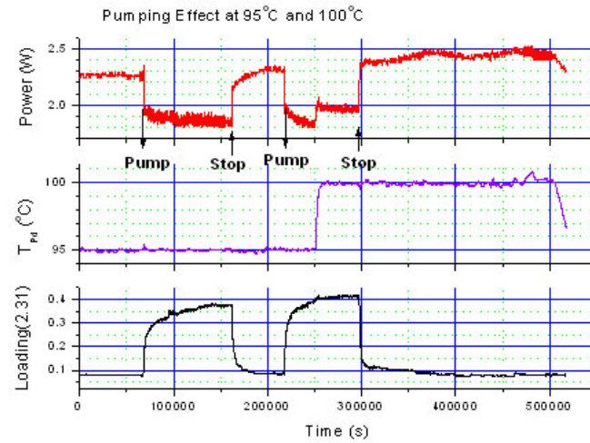
Figure 5. Excess heat under constant T_{pd} , 1998,12,13–17. (5_days7.xls).
