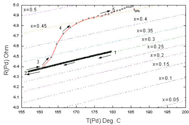
Figure 3. Pumping at 160°C induced a jump in loading ratio(constant current mode).
