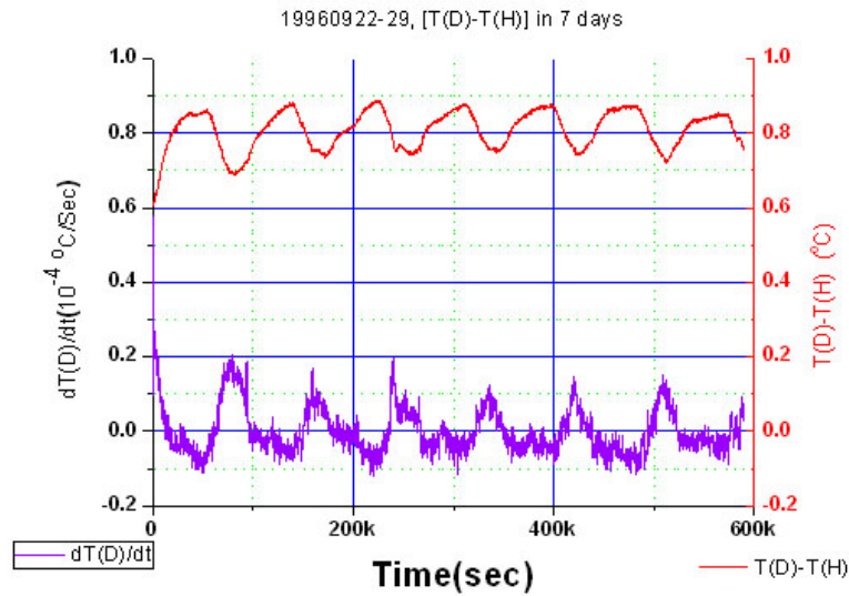
Figure 8. Temperature difference between D/Pd and H/Pd systems.
