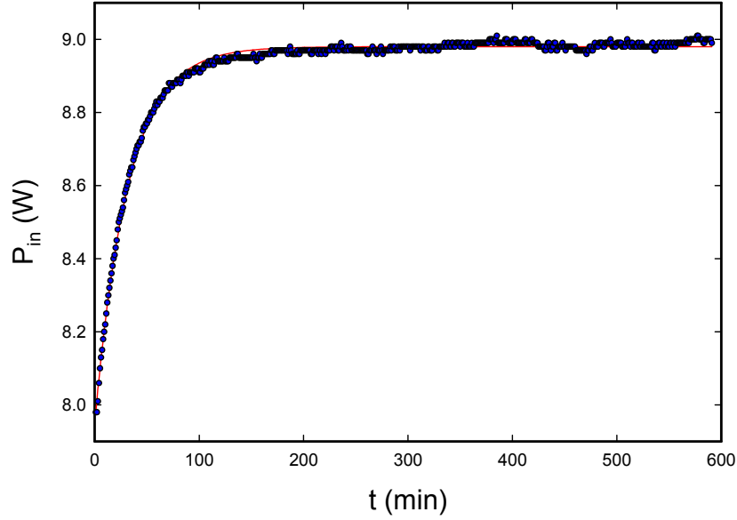
Figure 2. Output power points and fit for DGL662v2.
