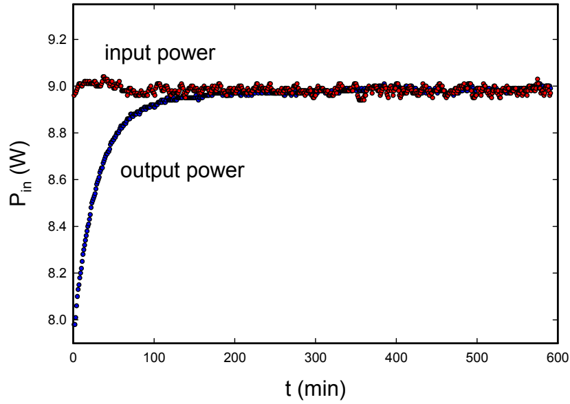
Figure 1. Input and output power points from DGL662v2.
