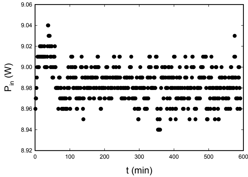
Figure 3. Input power points from DGL662v2.
