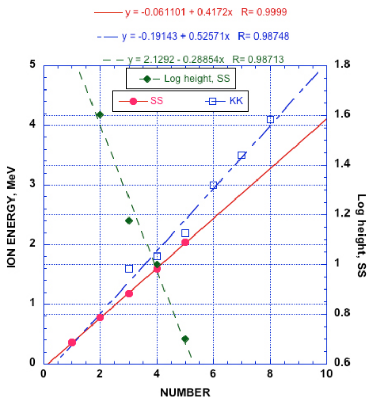
Figure 12. Comparison between the data sets in Figures 10 and 11. The log ion intensity is obtained from the data in Fig. 11. The first value in Fig. 10 is assumed to be point #3 in the sequence with the previous values being hidden in the noise.
