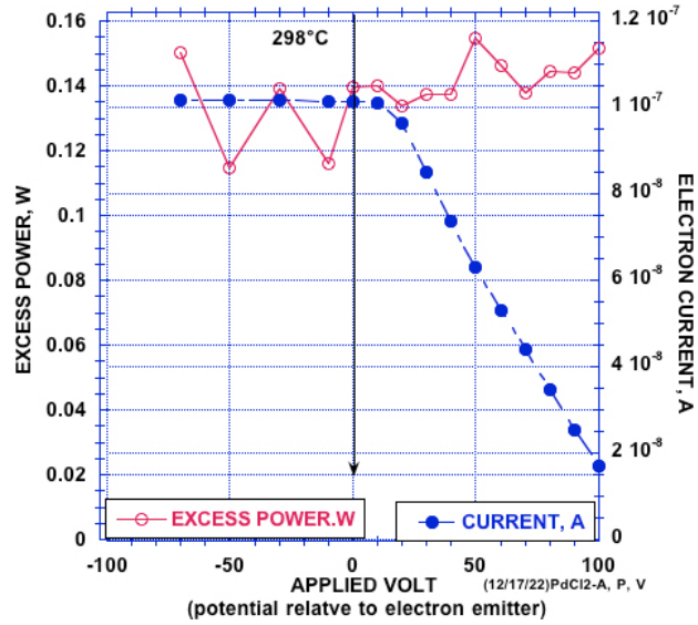
Figure 8. Effect of a voltage applied between the emitter and collector on the electron current at 298° C emitted from \alpha+\beta Pd in D 2 gas. The excess power is also shown.
