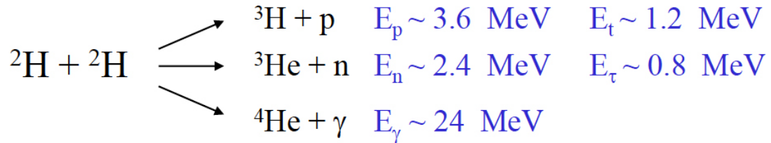
Figure 1. The energy of the emissions resulting from hot fusion between deuterons as provided by Czerski [3], [4]. The emission of {}^4\text{He} with a very energetic gamma ray has a very low probability. These reactions are never observed when cold fusion occurs.
