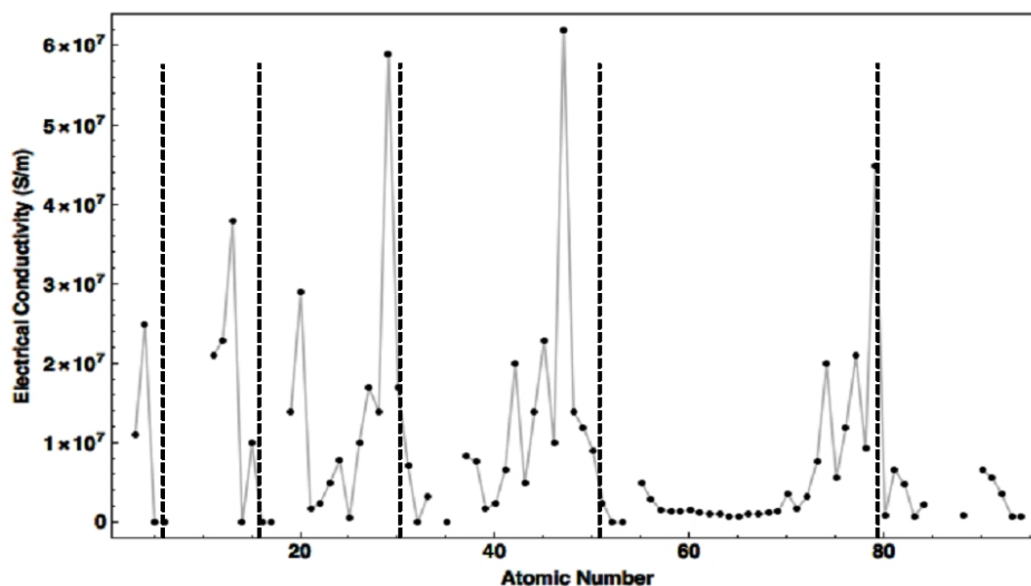
Figure 14. Compilation of the electrical conductivity in Siemens per meter (S/m) in solids of elements as a function of atomic number. The five dashed lines are at the same values of atomic number as in the earlier plots.
