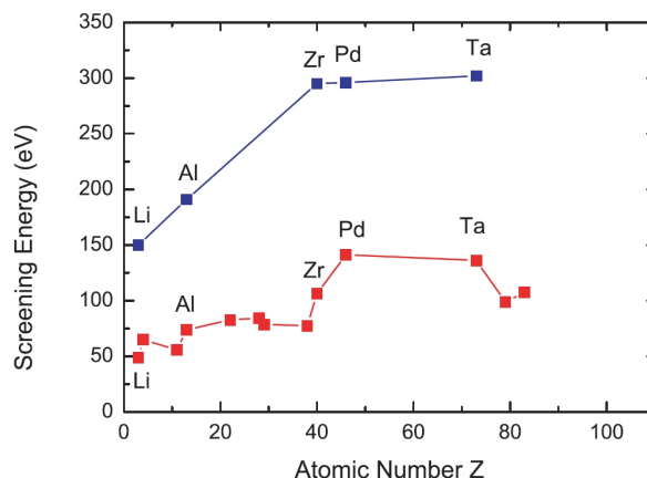
Figure 11. Screening potentials as a function of atomic number z . Top in blue: empirical values. Bottom in red: theoretical values.
