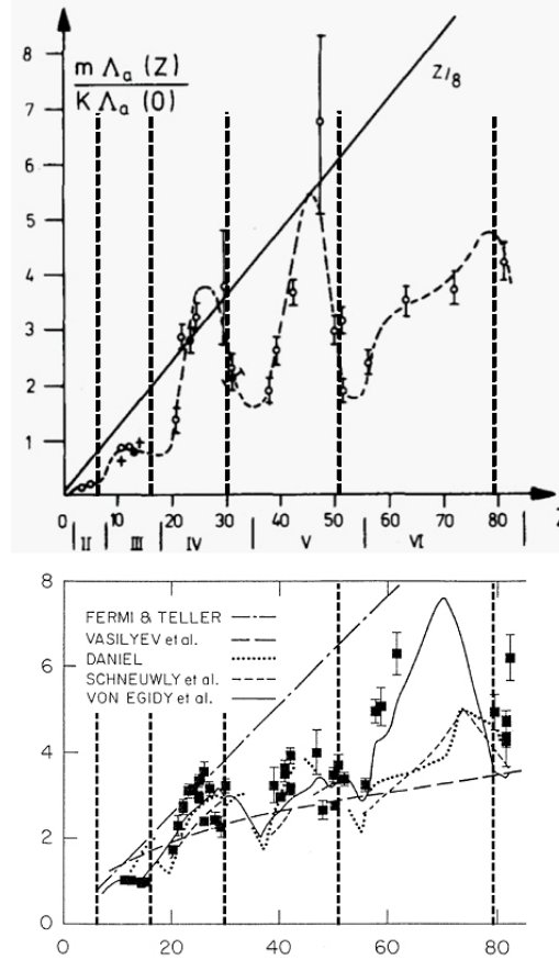
Figure 12. Top: “Periodicity of the relative atomic capture probability m\Delta_a(Z)/K\Delta_a(0) in metallic oxides Z_KO_m . Numerals II, . . . . VI represent the groups in the periodic table to which the metallic atoms belong.” The expectation of the Fermi-Teller law is represented by the straight line. Experimental data are from Zinov et al. Bottom: “Comparison of experimental and theoretical atomic capture ratios in oxides. The data are those of Stanislaus et al. The Fermi-Teller Z law is clearly inadequate as is the monotonic form of Vasilyev. Atomic structure is included in the calculations by Daniel, Schneuwly et al. , and von Egidy et al. , the theory with the best fit.” The vertical dashed lines in both plots occur at the same elements as in the earlier figures.
