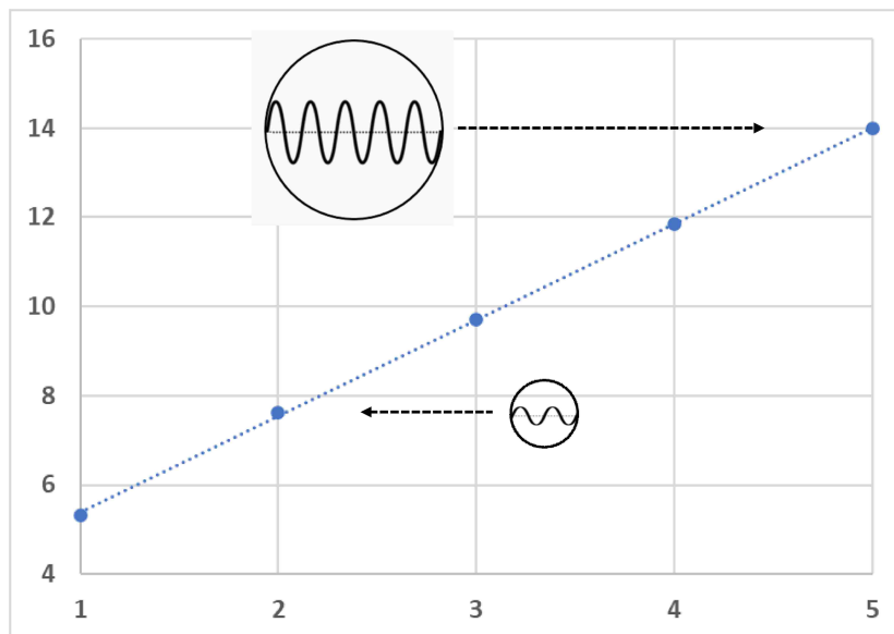
Figure 2. Relationship of the nuclear diameter D in femtometers vertically as a function of the numbers N of the peaks in Figure 1. The insets are cartoons of the fits for the second and fifth peaks. The equation for the line is D = 2.154 N + 3.234 with R^2 = 0.9998 . Hence, the plot gives the neutron wavelength in nuclear matter as 2.154 fm.
