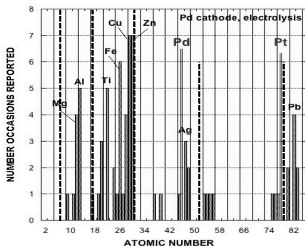
Figure 7. Histogram of the number of published papers and reports that claim the production of specific elements in LENR experiments, as labelled on this plot from Storms. The dashed lines correspond to the values of Z in the table above.
