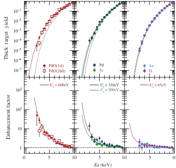
Figure 9. Top: Thick target fusion reaction yields for five different targets bombarded with deuterons at the indicated energies below 10 keV. The yields are normalized to unity at 10 keV. The dashed lines are extrapolations of the curves for higher impact energies. Bottom: Ratios of the measured and extrapolated yield values, with computed ratios for different screening potentials noted in the figure (solid lines).
