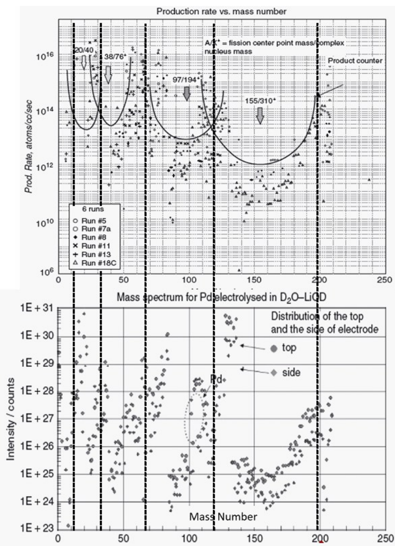
Figure 6. Transmutation data as a function of atomic mass A in AMU. Top: Absolute elemental production rate in atoms per cubic centimeter per second from Miley and Patterson. Bottom: Count rate from mass spectrometry measurements by Mizuno, Ohmori and Enyo. The vertical dashed lines are at atomic mass numbers that are the same as the peaks in Figure 1.
