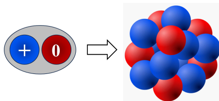
Figure 13. Deuteron on the left, with its oriented proton and neutron, approaching a target nucleus.
