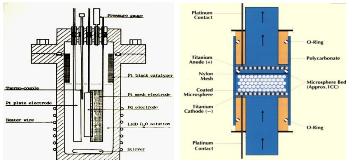
Figure 4. Left: A schematic of the experiment by Mizuno, Ohmori and Enyo. Right: A drawing of the experiments by Miley and Patterson, which was similar to that used by Little and Puthoff.
