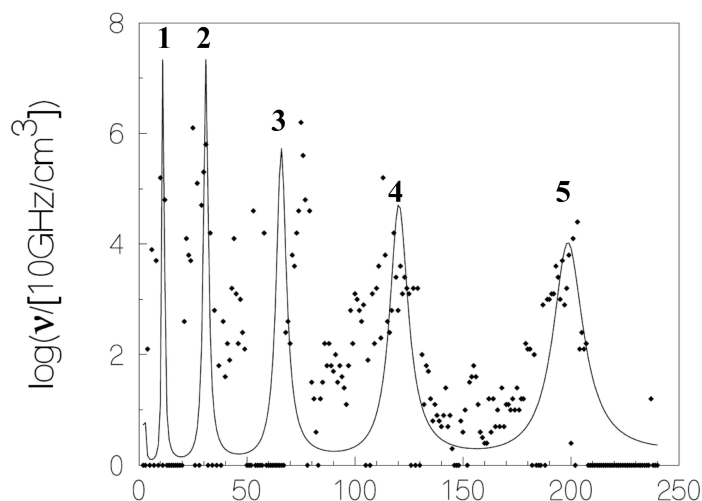
Figure 1. Plot of the nuclear rate in reactions per second per cubic centimeter measured by Miley and Patterson (the points) and the Widom-Larsen theoretical optical model f(A) multiplied by four (the line) versus atomic mass number. The peaks are numbered sequentially.
