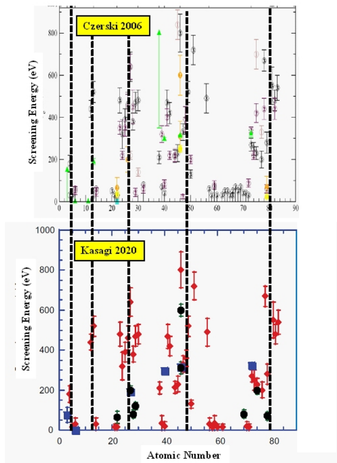
Figure 10. Compilations of empirical screening potentials for deuteron fusion as a function of the atomic number of the target material in which they were measured. The five dashed lines are at the same values of atomic size as in the earlier plots.
