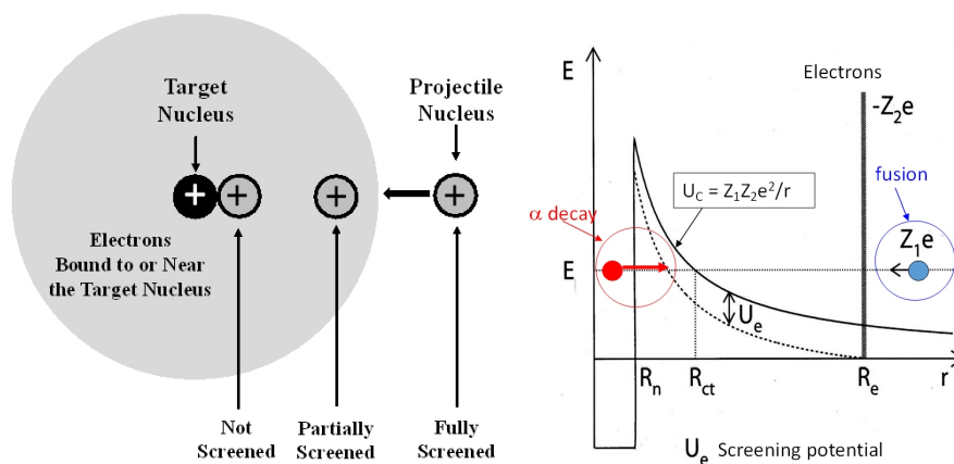
Figure 8. Left: Schematic of the projectile nucleus positions at three times before a nuclear collision. The nuclei are shown as 1/10 of the atomic size. In reality, the nuclei are 1/100,000 the size of an atom. Right: Schematic by Kasagi of the kinetic and potential energies for (a) an incident projectile with charge Z_1 e (blue) prior to a fusion reaction, and (b) an alpha particle escaping from a radioactive or other nucleus (red). Both are at “sub-Coulomb” energies, that is, below the maximum of the Coulomb potential at the nuclear boundary R_n .
