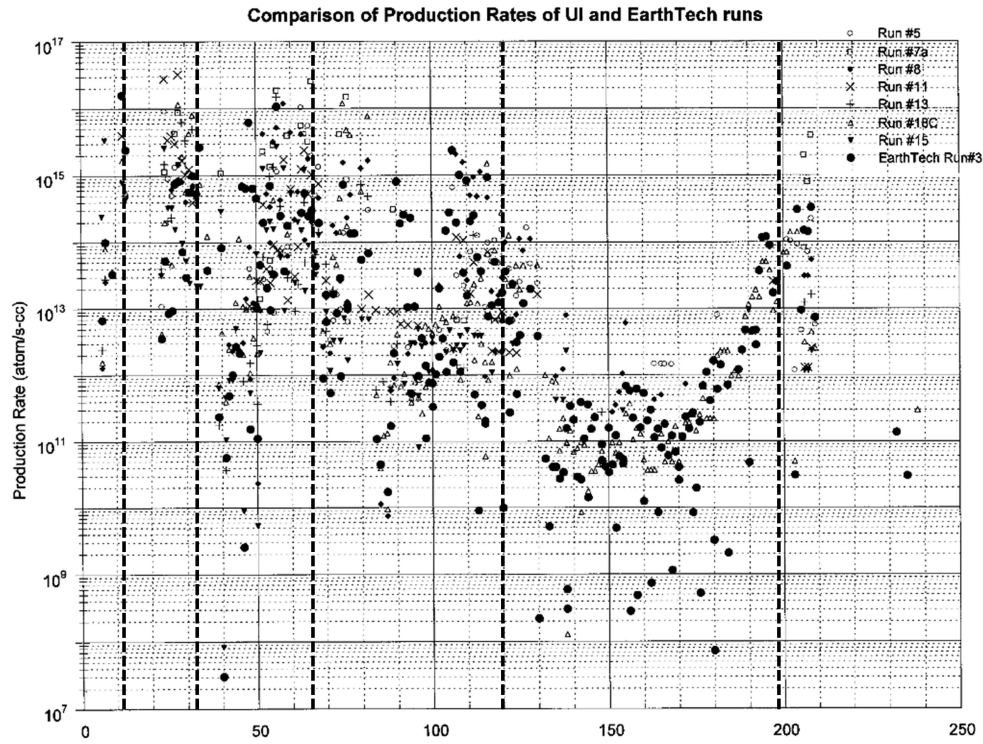
Figure 5. Overplot of the transmutation results from EarthTech run #3 by Little and Puthoff (heavy black dots) with the data from seven runs by Miley and Patterson (other symbols). The vertical dashed lines are at the positions of the peaks in the Optical Model, as shown in Figure 1.
