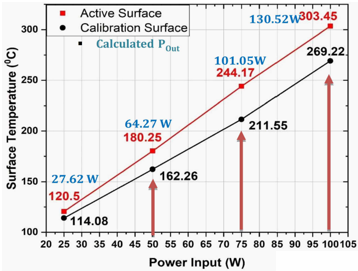
Graph 1. Graph of Surface Temperature (°C) Vs Power input (W). The calculated power output for the active experiments also mentioned in the graph (quantification done by comparing with the data of calibration experiment).
