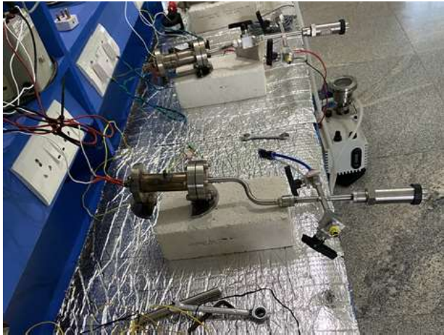
Figure 2. Parallel experiment setup.
